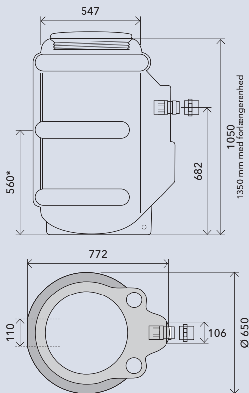
Micro 5G/7G, tegning (mm)
